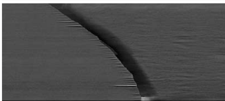
Bediener Software
